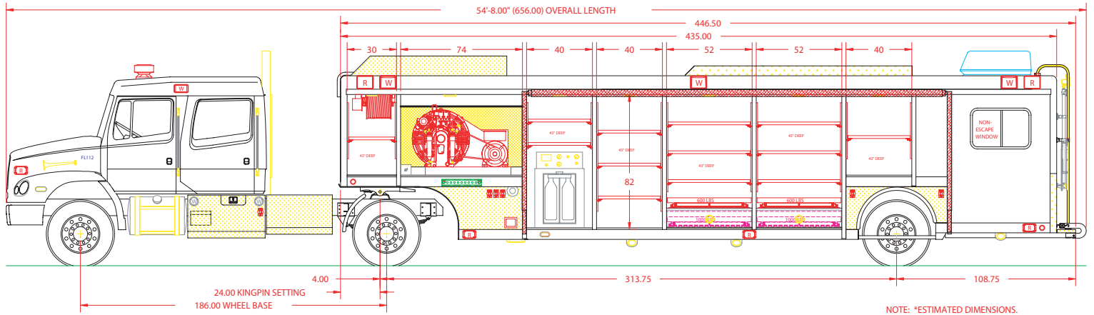
ROADSIDE (OBSERV. PLATFORM SHOWN WITH RAILS IN DOWN POSITION)
