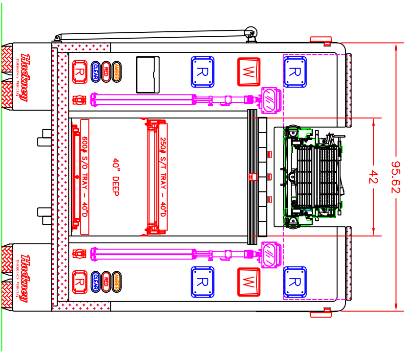
REAR VIEW (SHOWN W/ADS IN STOWED POSITION)
