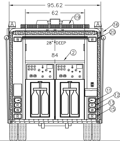
REAR END VIEW
