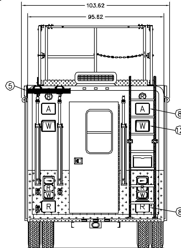
REAR VIEW (OBSERV. PLATFORM SHOWN WITH RAILS IN UP POSITION)
