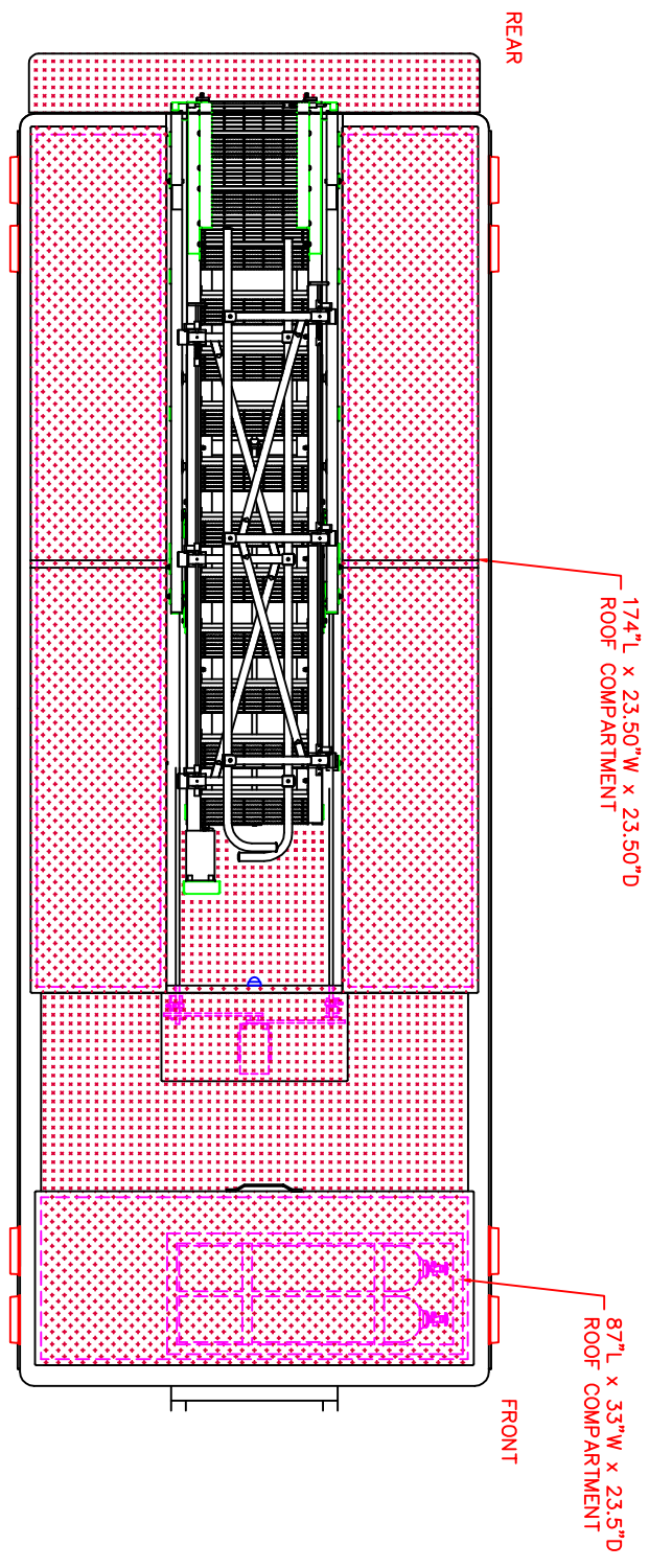
TOP PLAN VIEW (SHOWN WITH ADS STAIRCASE IN STOWED POSITION)
